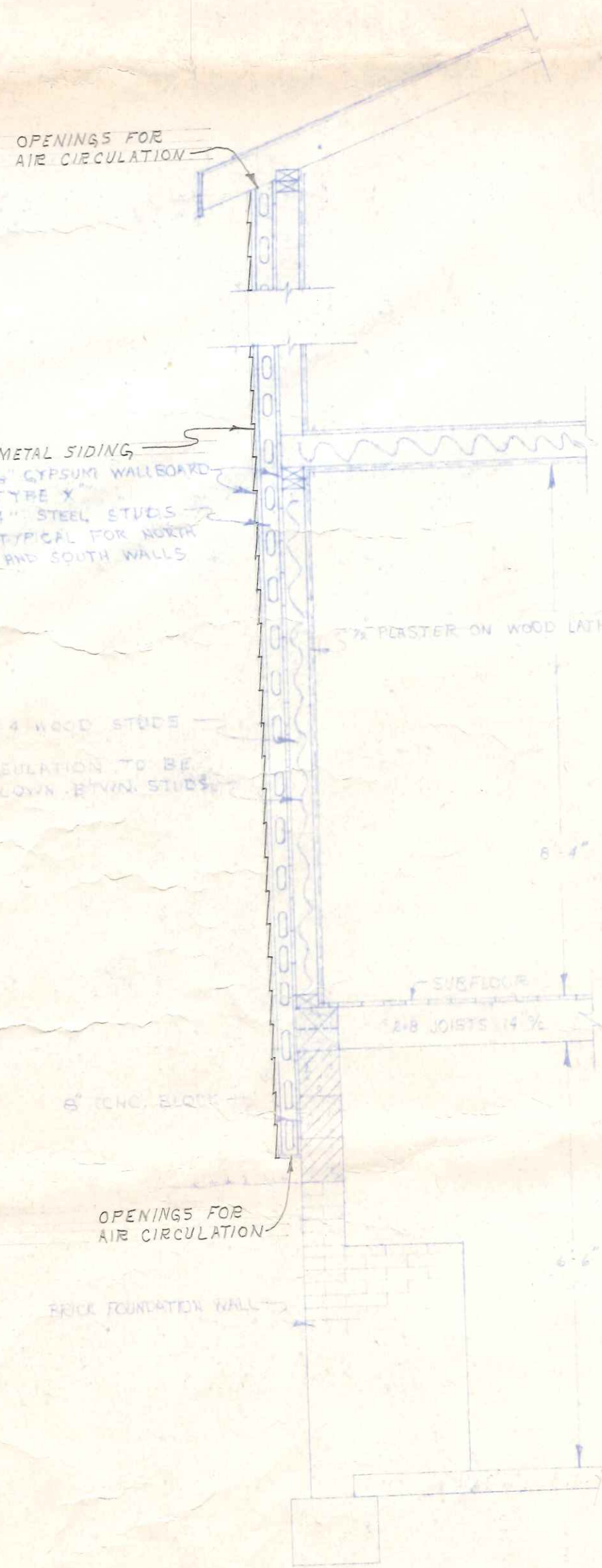
WALL DETAIL SCALE 1/4" = 1'-0"
