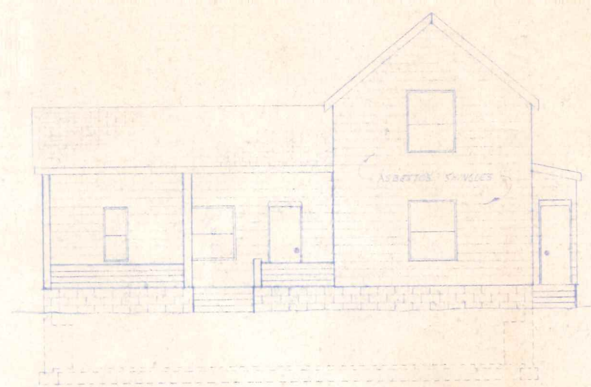
EAST ELEVATION SCALE 1/4" = 1'-0"
